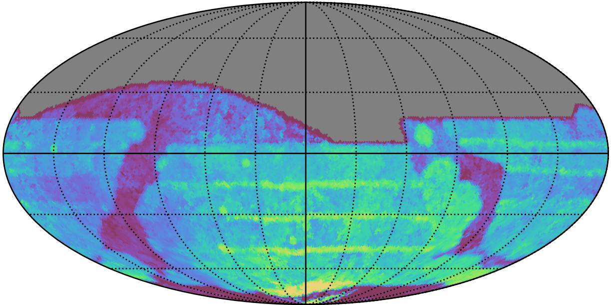
too_elab_heavy_r64_d2_ugrizy_v3.4_10yrs All sky all bands: Median Season Length
