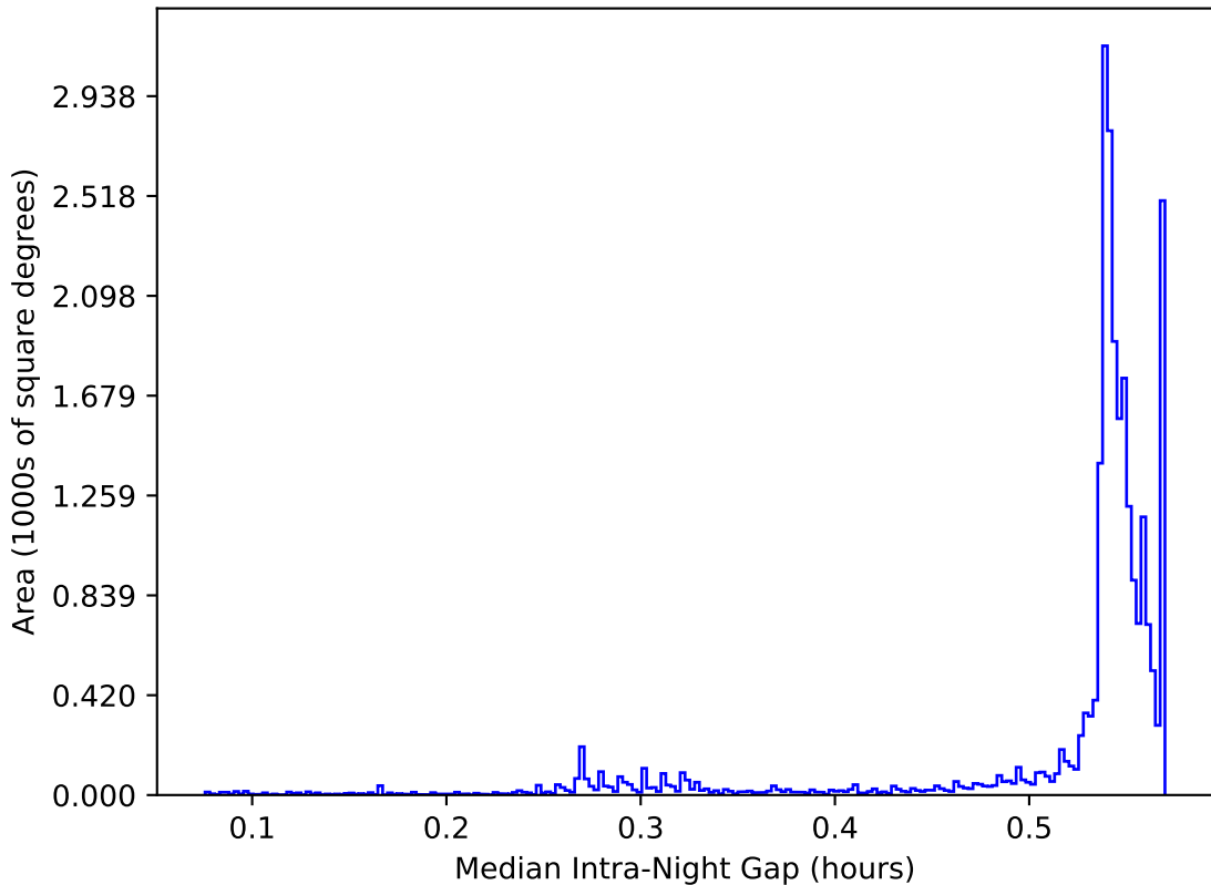
too_elab_heavy_r64_d2_ugrizy_v3.4_10yrs All sky: Median Intra-Night Gap
