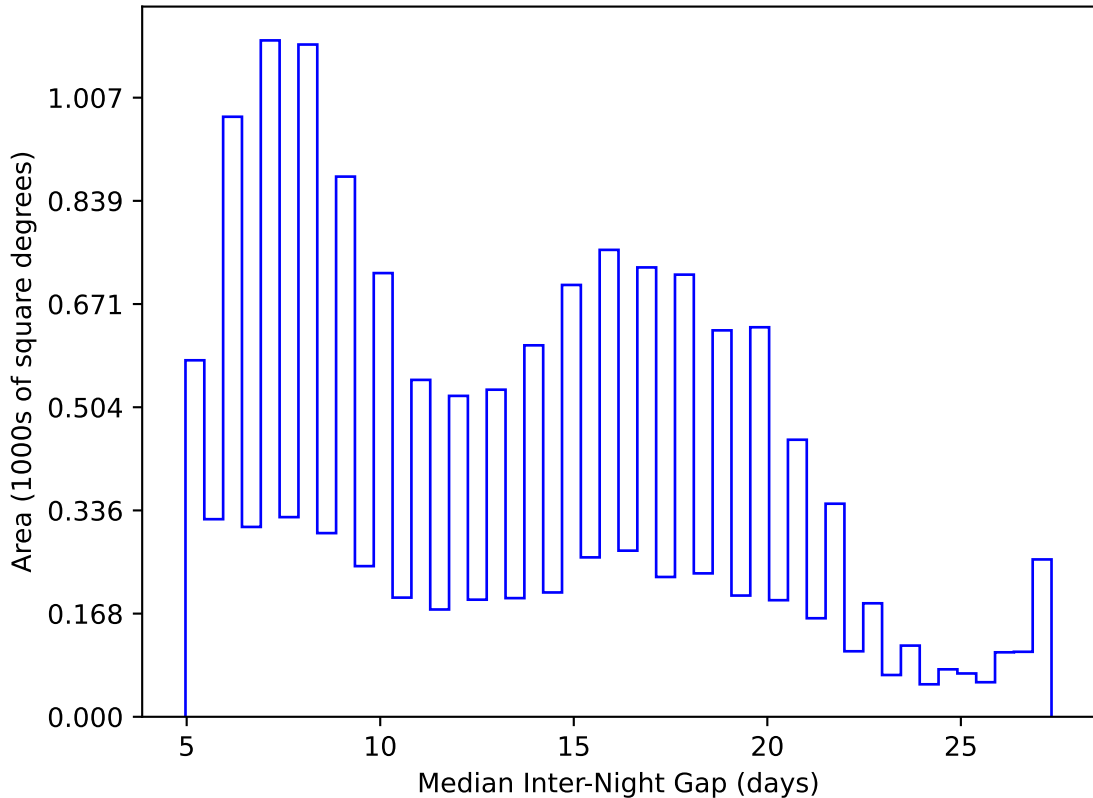
too_elab_heavy_r64_d2_ugrizy_v3.4_10yrs WFD y band: Median Inter-Night Gap
