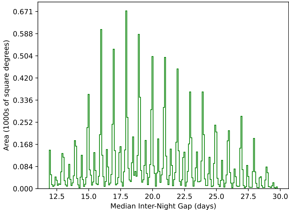
too_elab_heavy_r64_d2_ugrizy_v3.4_10yrs WFD g band: Median Inter-Night Gap
