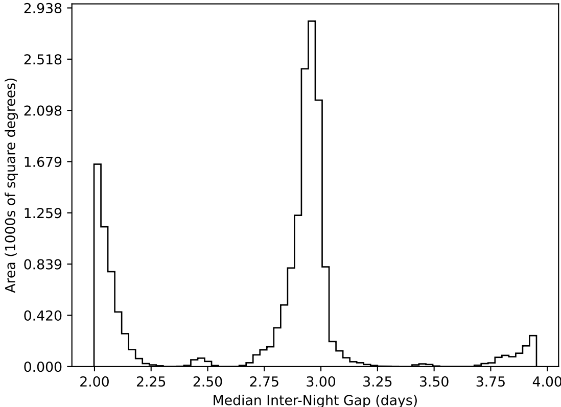
too_elab_heavy_r64_d2_ugrizy_v3.4_10yrs WFD all bands: Median Inter-Night Gap
