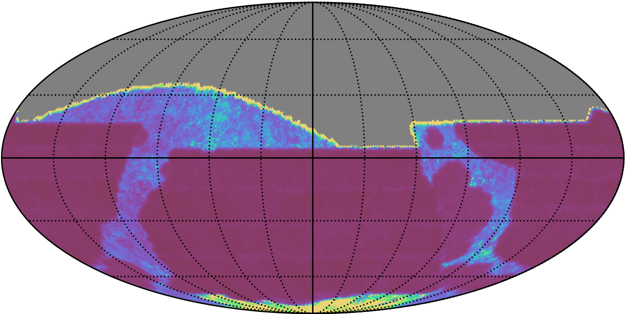
too_elab_heavy_r64_d2_ugrizy_v3.4_10yrs All sky i band: Median Inter-Night Gap
