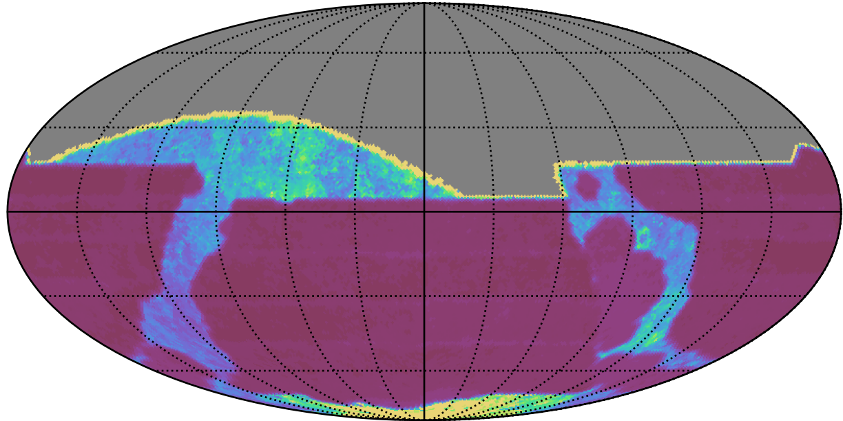
too_elab_heavy_r64_d2_ugrizy_v3.4_10yrs All sky all bands: Median Inter-Night Gap
