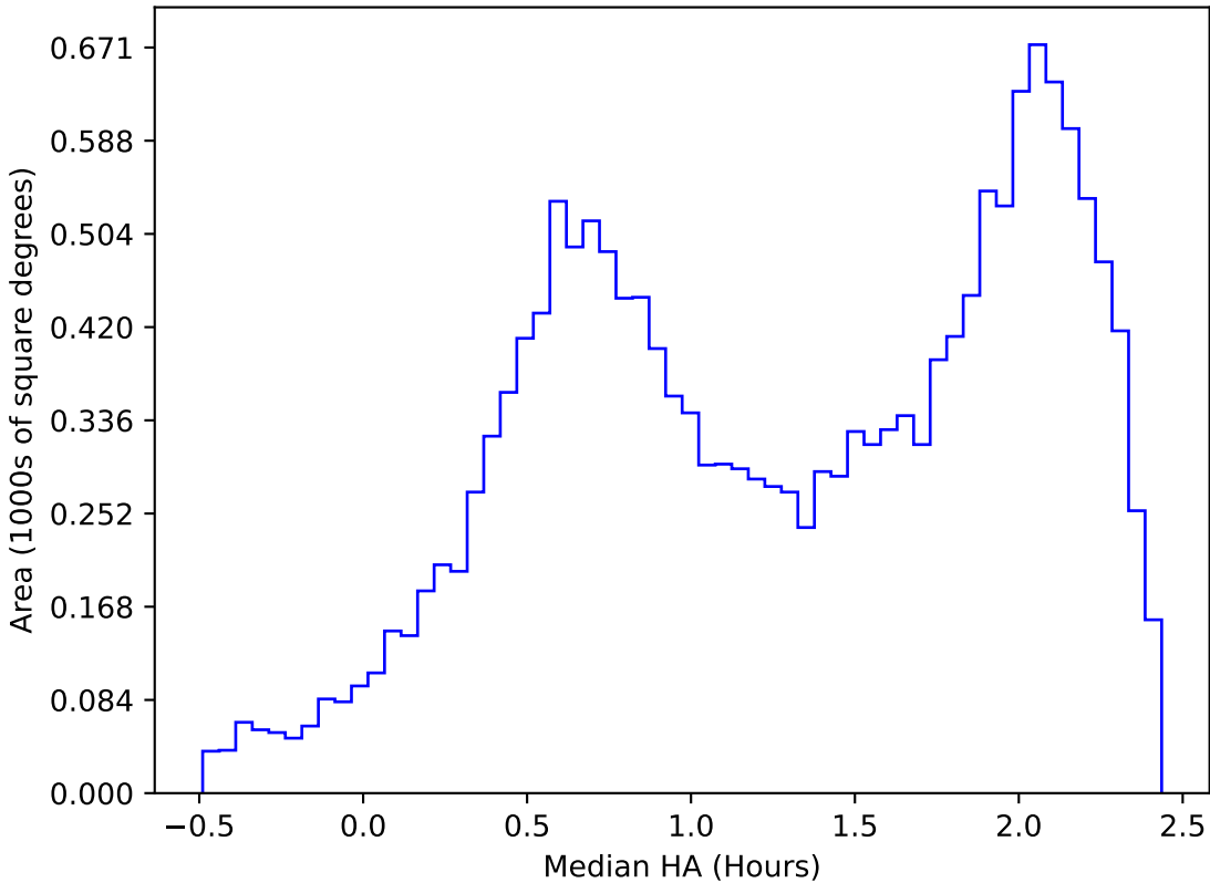
too_elab_heavy_r64_d2_ugrizy_v3.4_10yrs WFD y band: Median HA
