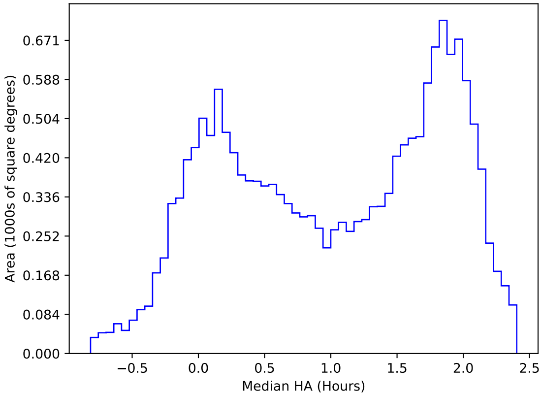
too_elab_heavy_r64_d2_ugrizy_v3.4_10yrs WFD u band: Median HA
