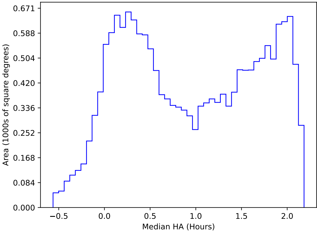
too_elab_heavy_r64_d2_ugrizy_v3.4_10yrs WFD r band: Median HA
