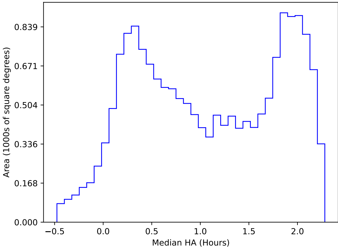
too_elab_heavy_r64_d2_ugrizy_v3.4_10yrs WFD i band: Median HA
