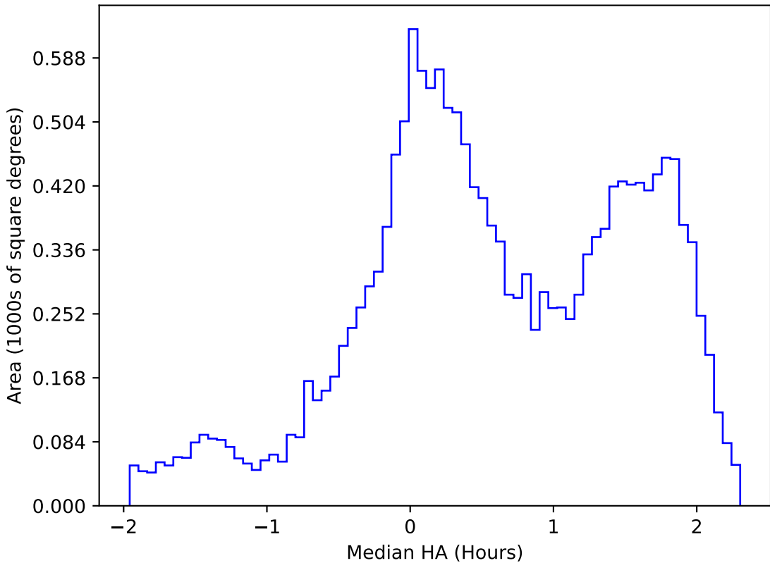
too_elab_heavy_r64_d2_ugrizy_v3.4_10yrs WFD g band: Median HA
