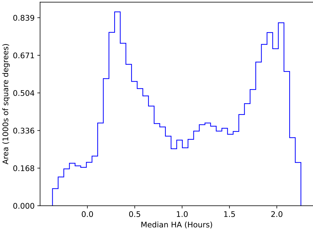
too_elab_heavy_r64_d2_ugrizy_v3.4_10yrs WFD all bands: Median HA
