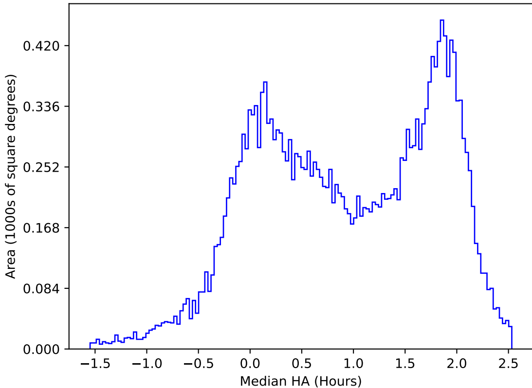
too_elab_heavy_r64_d2_ugrizy_v3.4_10yrs All sky u band: Median HA
