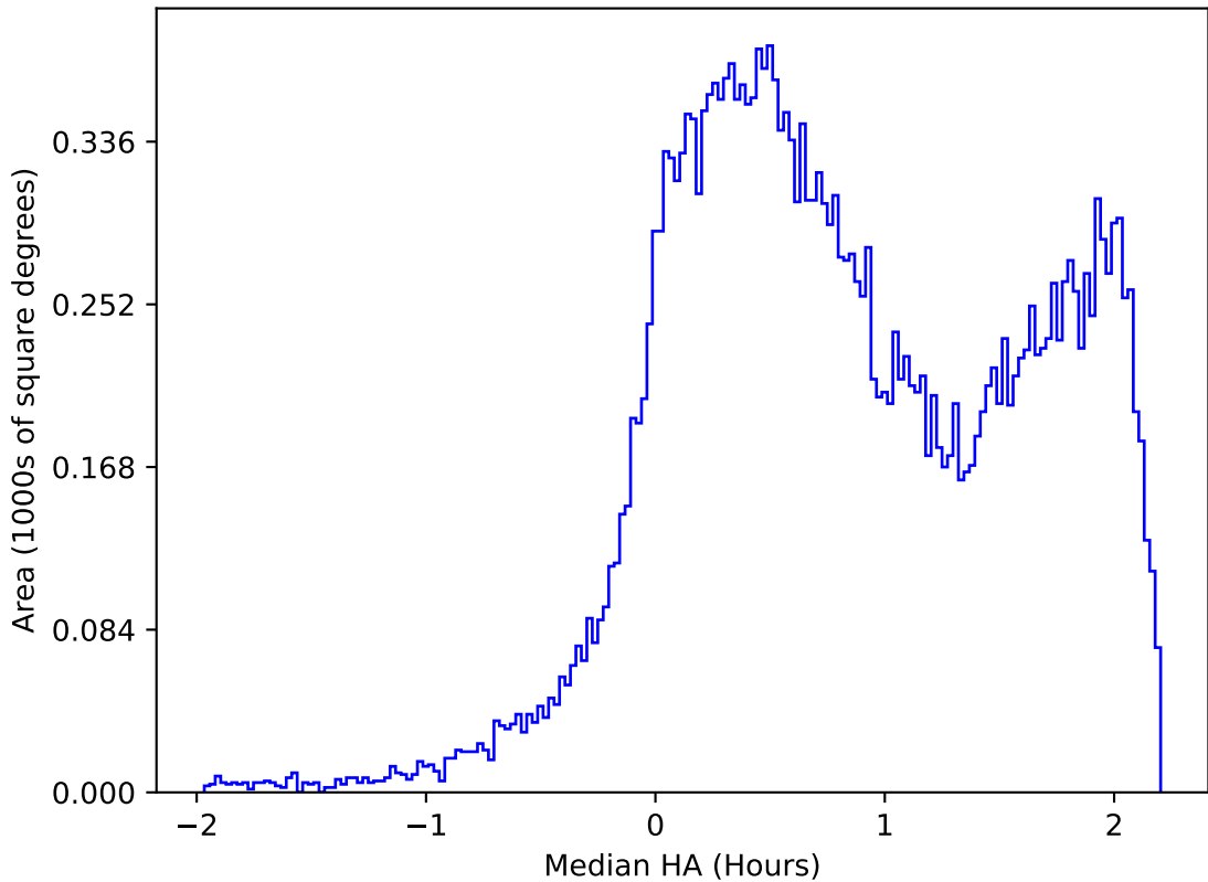
too_elab_heavy_r64_d2_ugrizy_v3.4_10yrs All sky r band: Median HA
