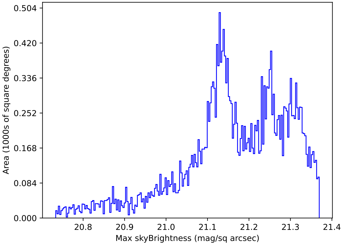
too_elab_heavy_r64_d2_ugrizy_v3.4_10yrs Yr 1 r band: Max skyBrightness
