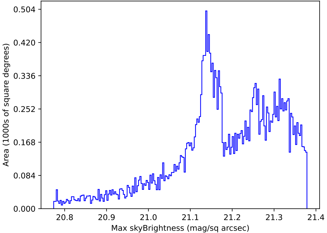
too_elab_heavy_r64_d2_ugrizy_v3.4_10yrs All sky r band: Max skyBrightness
