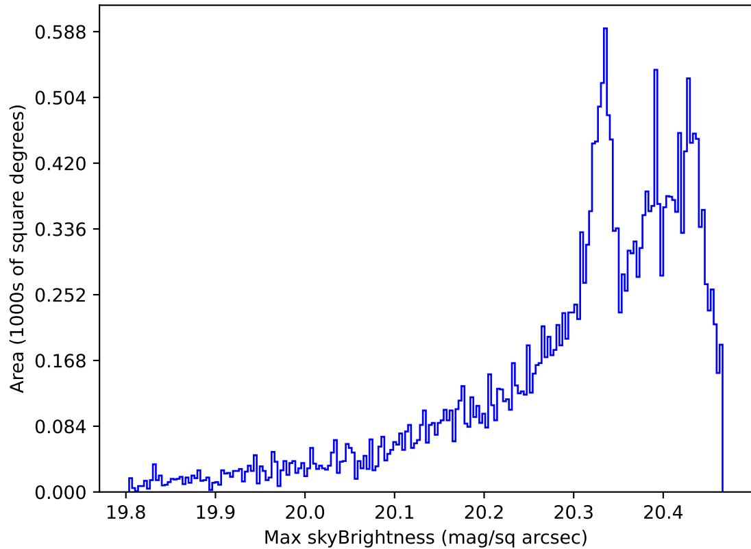
too_elab_heavy_r64_d2_ugrizy_v3.4_10yrs All sky i band: Max skyBrightness
