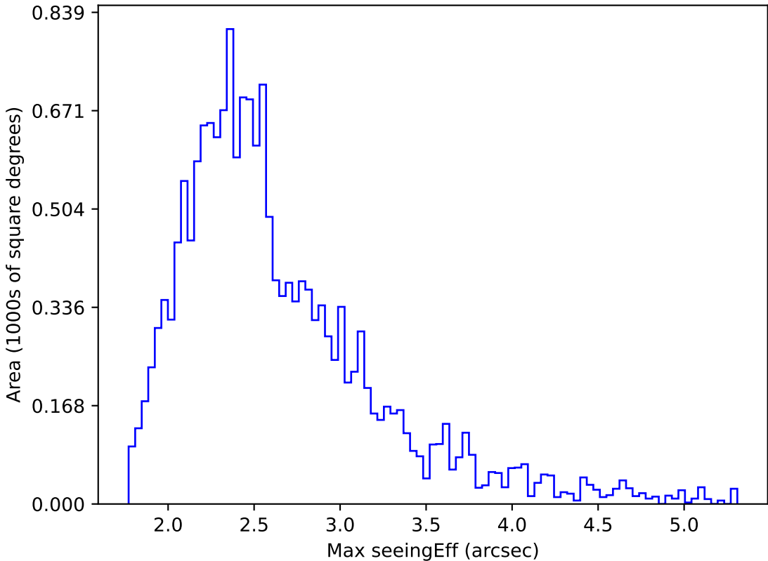
too_elab_heavy_r64_d2_ugrizy_v3.4_10yrs WFD i band: Max seeingEff
