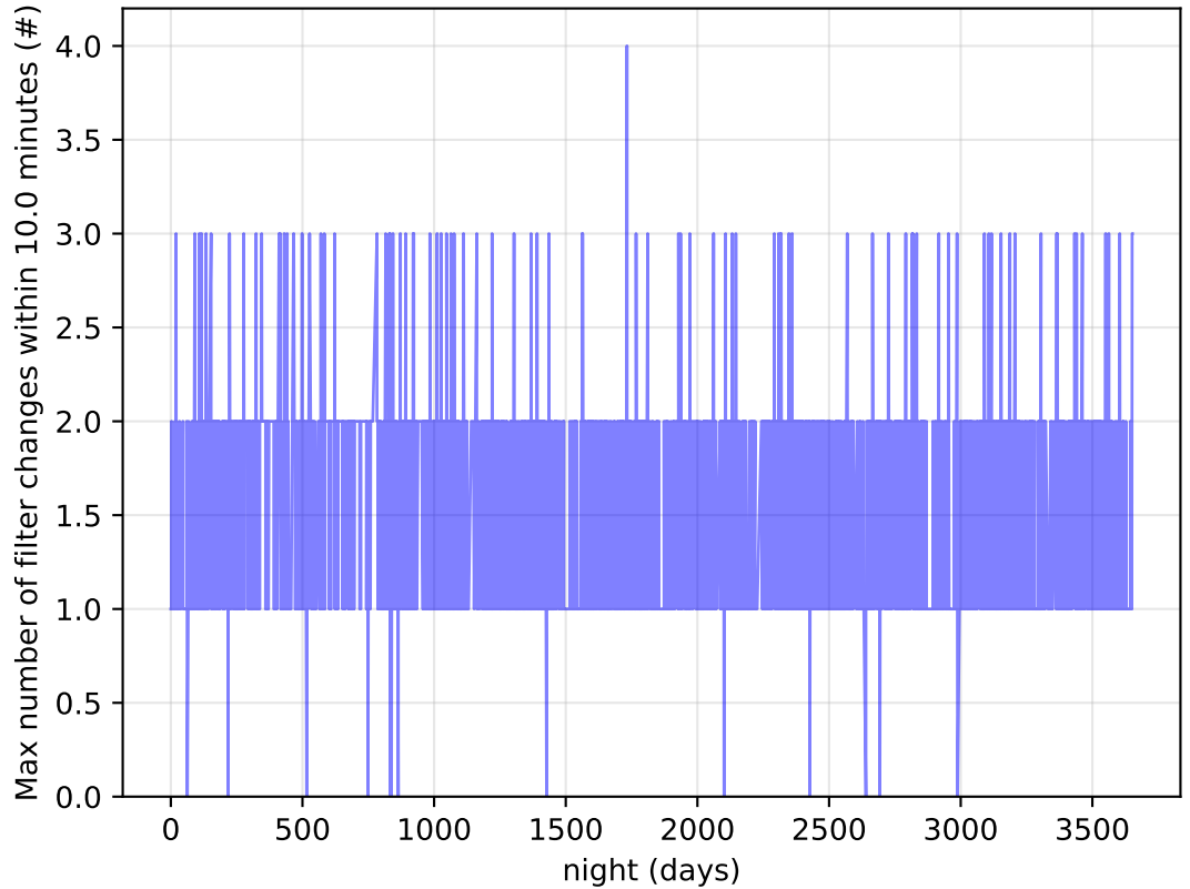
too_elab_heavy_r64_d2_ugrizy_v3.4_10yrs Per Night: Max number of filter changes within 10.0 minutes
