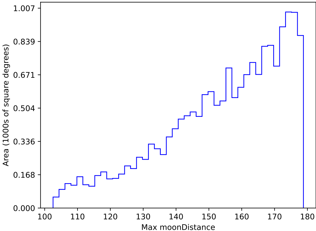
too_elab_heavy_r64_d2_ugrizy_v3.4_10yrs WFD g band: Max moonDistance
