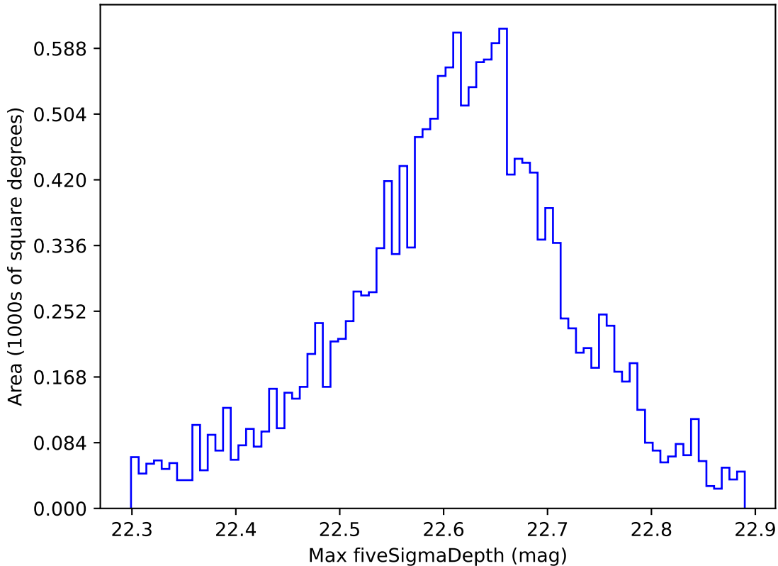
too_elab_heavy_r64_d2_ugrizy_v3.4_10yrs WFD y band: Max fiveSigmaDepth
