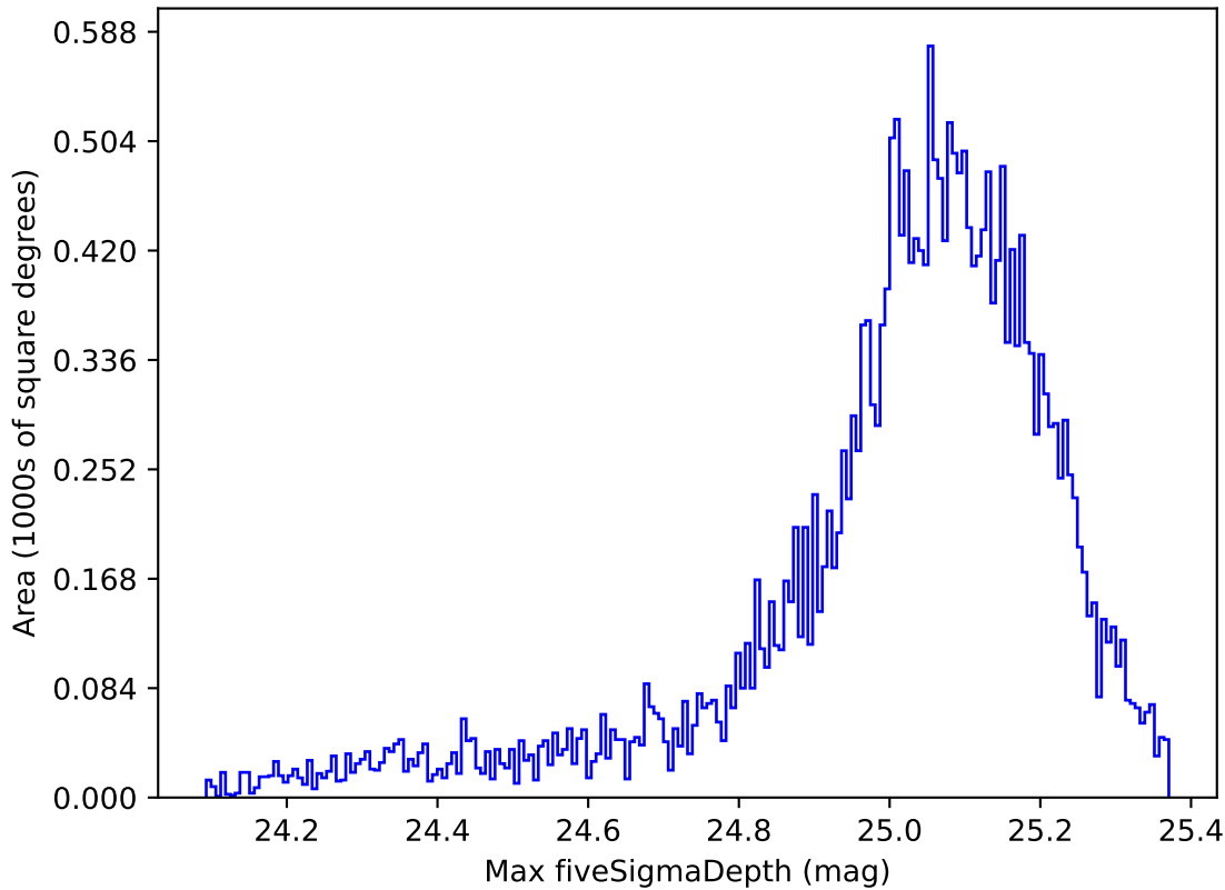
too_elab_heavy_r64_d2_ugrizy_v3.4_10yrs All sky all bands: Max fiveSigmaDepth
