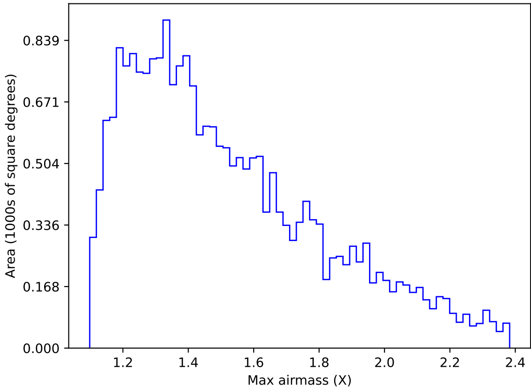
too_elab_heavy_r64_d2_ugrizy_v3.4_10yrs Yr 1 u band: Max airmass
