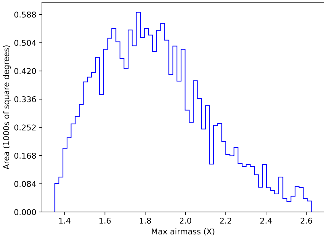
too_elab_heavy_r64_d2_ugrizy_v3.4_10yrs WFD u band: Max airmass
