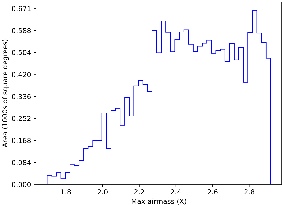
too_elab_heavy_r64_d2_ugrizy_v3.4_10yrs WFD i band: Max airmass
