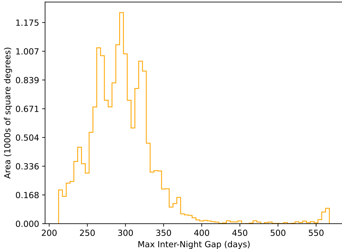
too_elab_heavy_r64_d2_ugrizy_v3.4_10yrs WFD r band: Max Inter-Night Gap
