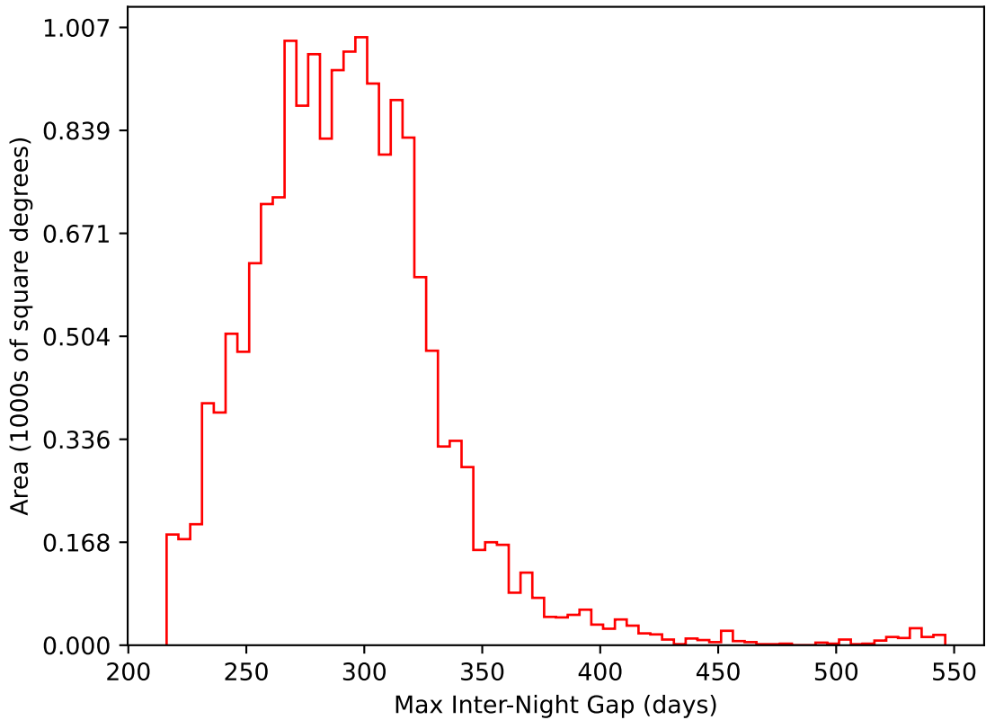
too_elab_heavy_r64_d2_ugrizy_v3.4_10yrs WFD i band: Max Inter-Night Gap
