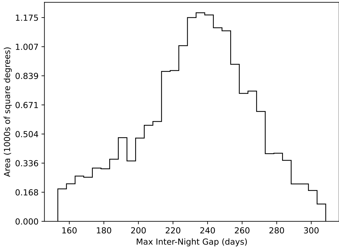
too_elab_heavy_r64_d2_ugrizy_v3.4_10yrs WFD all bands: Max Inter-Night Gap
