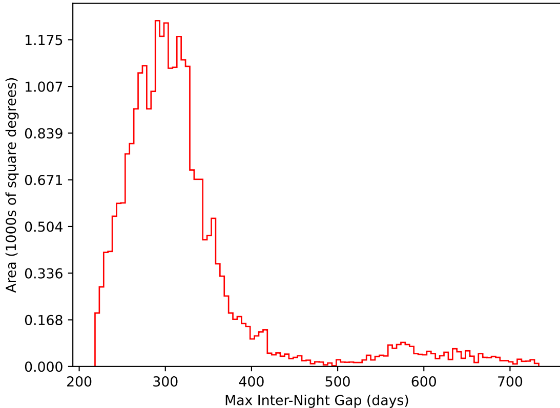
too_elab_heavy_r64_d2_ugrizy_v3.4_10yrs All sky i band: Max Inter-Night Gap
