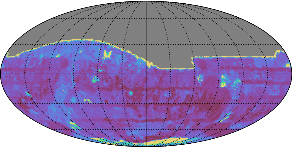
too_elab_heavy_r64_d2_ugrizy_v3.4_10yrs All sky all bands: Max Inter-Night Gap
