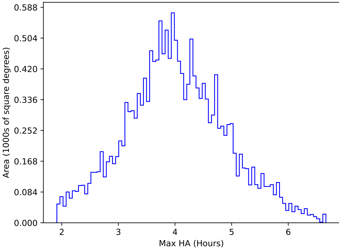
too_elab_heavy_r64_d2_ugrizy_v3.4_10yrs WFD u band: Max HA
