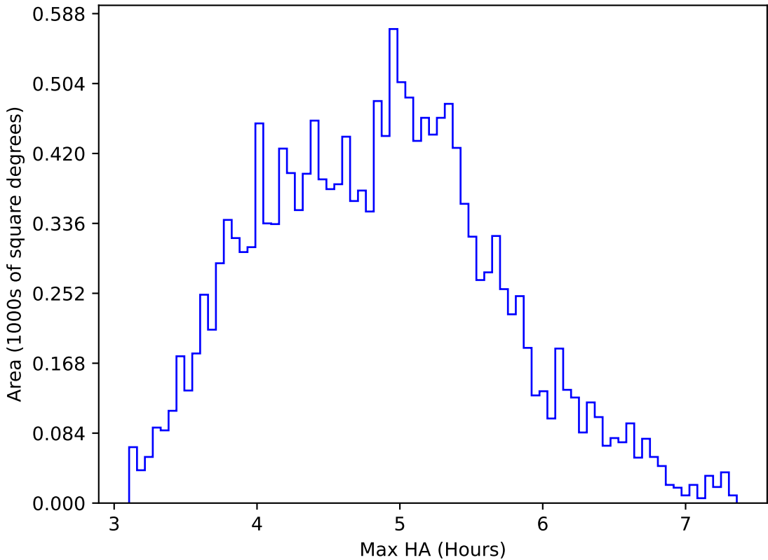
too_elab_heavy_r64_d2_ugrizy_v3.4_10yrs WFD i band: Max HA
