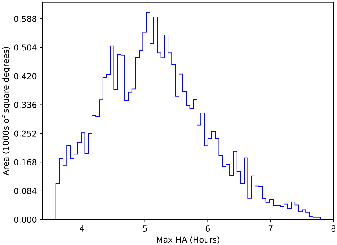
too_elab_heavy_r64_d2_ugrizy_v3.4_10yrs WFD all bands: Max HA
