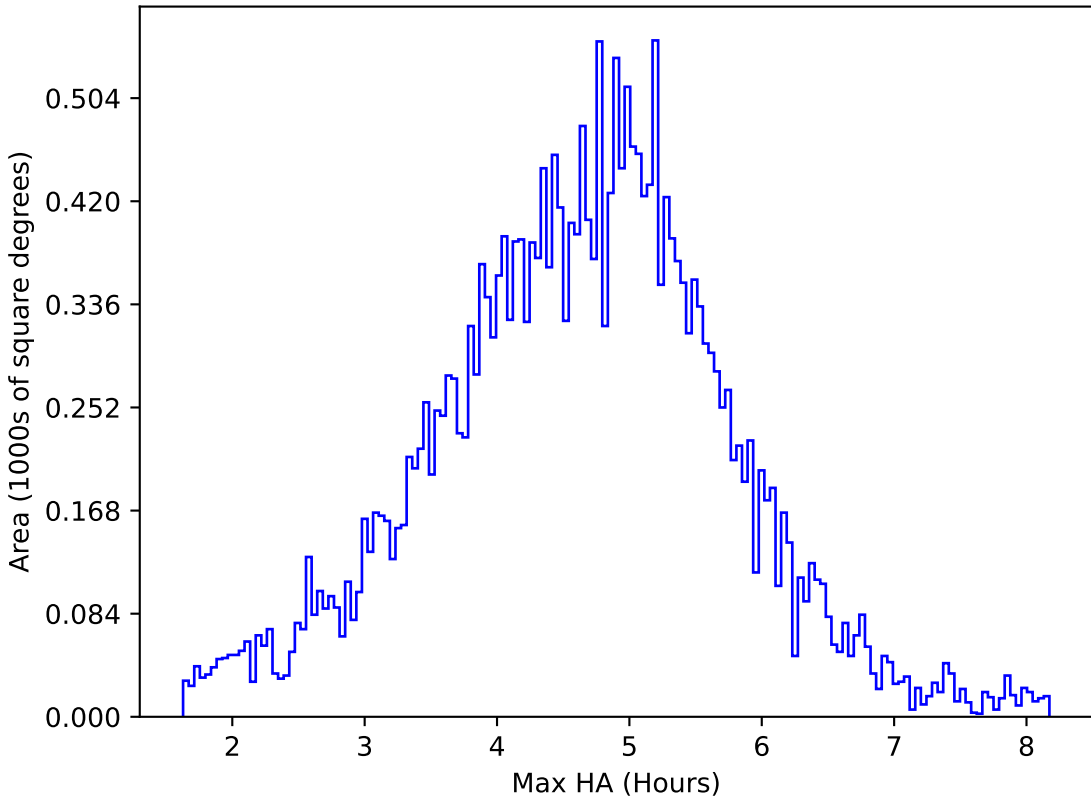
too_elab_heavy_r64_d2_ugrizy_v3.4_10yrs All sky z band: Max HA
