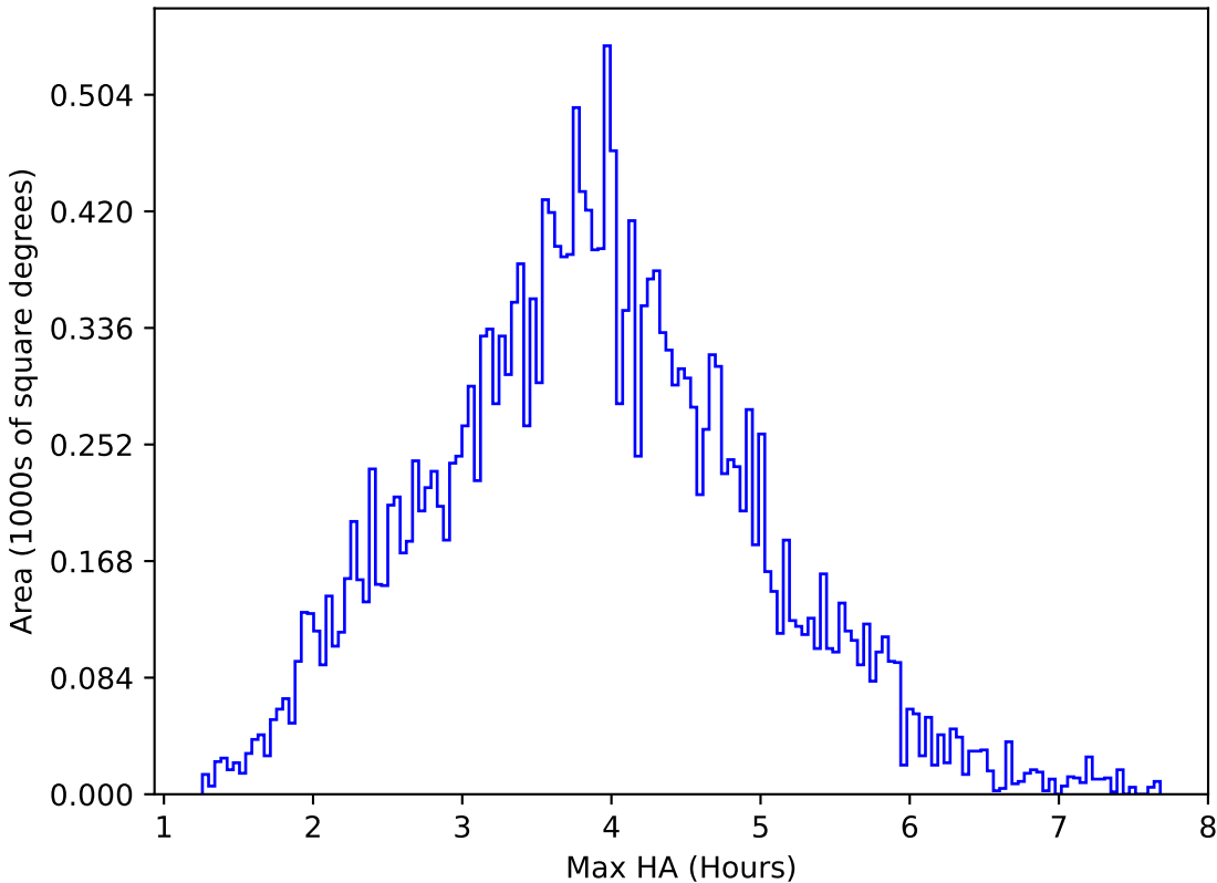
too_elab_heavy_r64_d2_ugrizy_v3.4_10yrs All sky u band: Max HA
