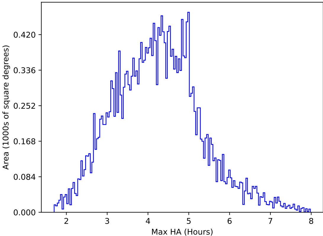
too_elab_heavy_r64_d2_ugrizy_v3.4_10yrs All sky r band: Max HA
