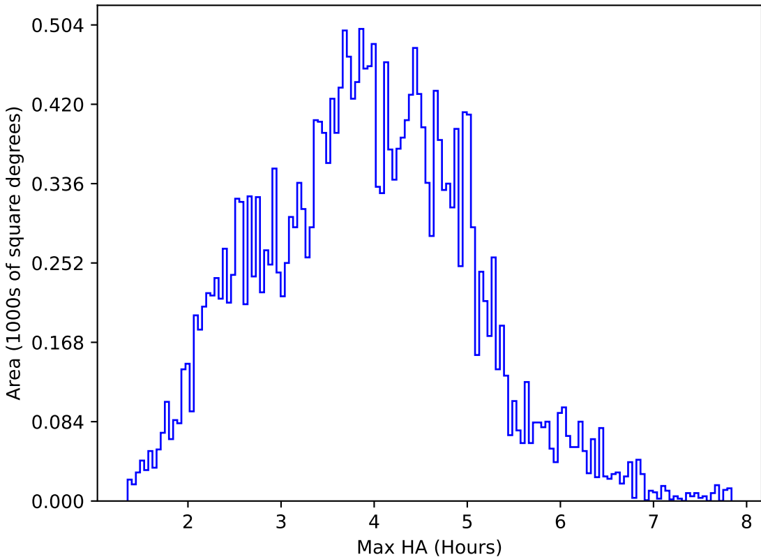
too_elab_heavy_r64_d2_ugrizy_v3.4_10yrs All sky g band: Max HA
