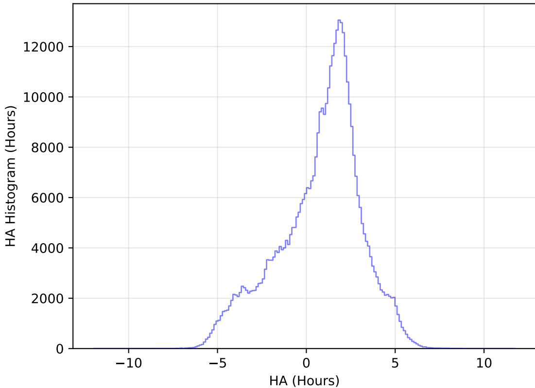
too_elab_heavy_r64_d2_ugrizy_v3.4_10yrs WFD z band: HA Histogram
