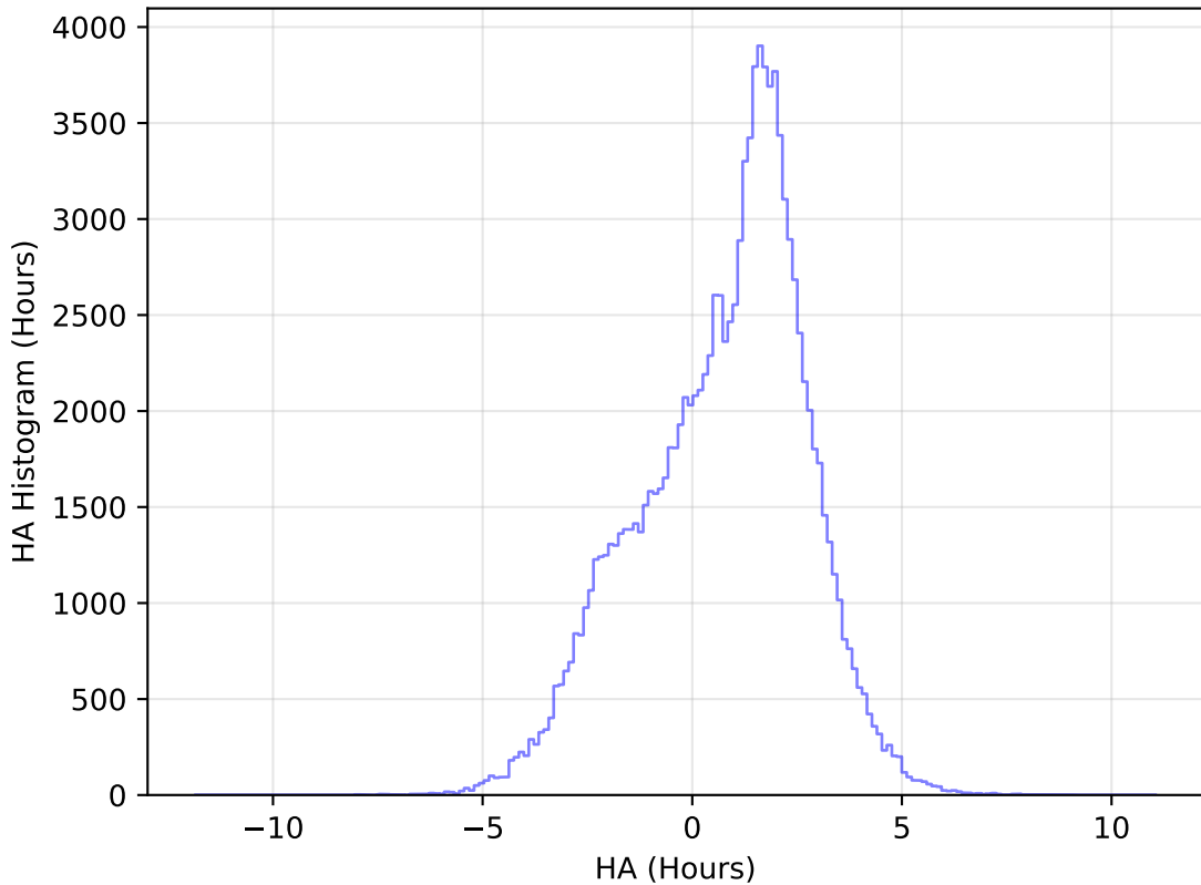
too_elab_heavy_r64_d2_ugrizy_v3.4_10yrs WFD u band: HA Histogram
