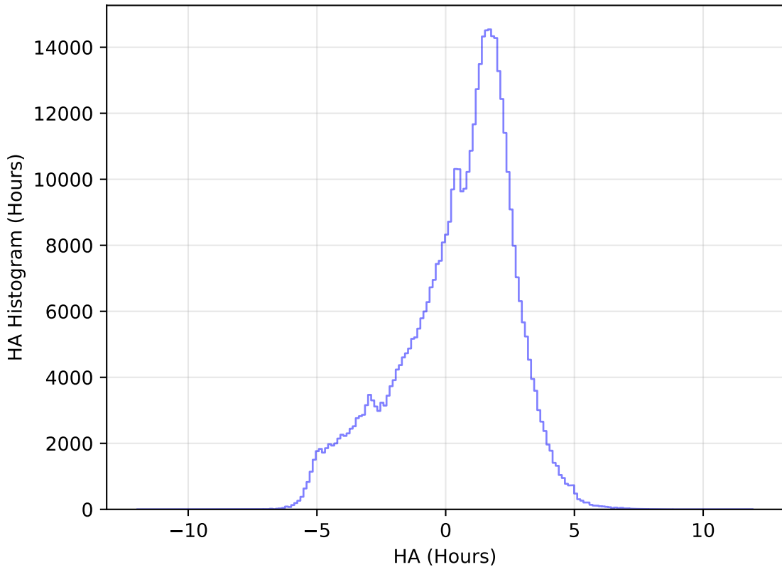
too_elab_heavy_r64_d2_ugrizy_v3.4_10yrs WFD r band: HA Histogram
