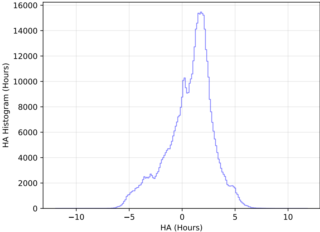
too_elab_heavy_r64_d2_ugrizy_v3.4_10yrs WFD i band: HA Histogram
