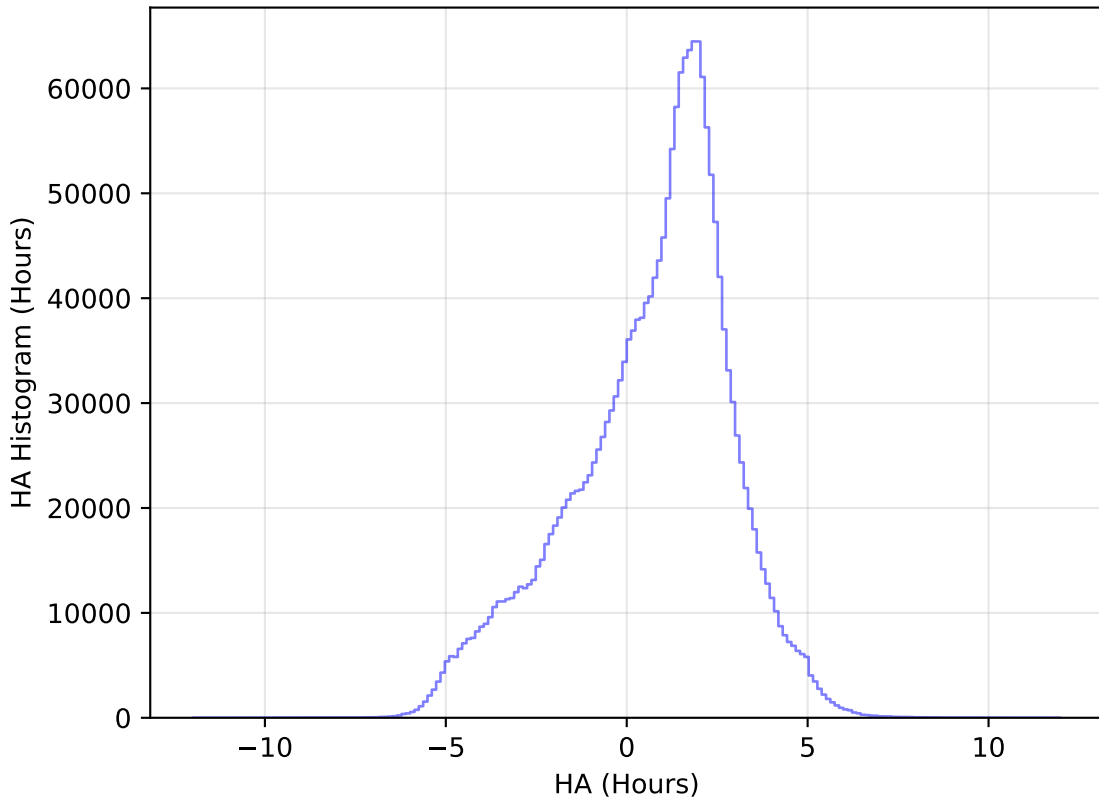
too_elab_heavy_r64_d2_ugrizy_v3.4_10yrs WFD all bands: HA Histogram
