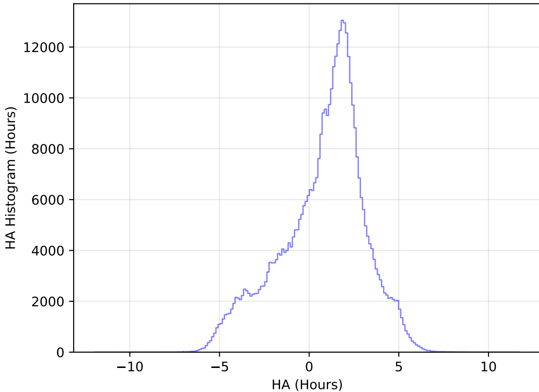
too_elab_heavy_r64_d2_ugrizy_v3.4_10yrs All sky z band: HA Histogram
