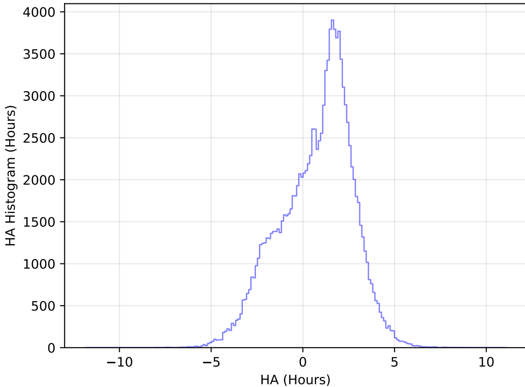
too_elab_heavy_r64_d2_ugrizy_v3.4_10yrs All sky u band: HA Histogram
