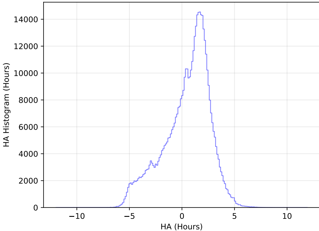
too_elab_heavy_r64_d2_ugrizy_v3.4_10yrs All sky r band: HA Histogram
