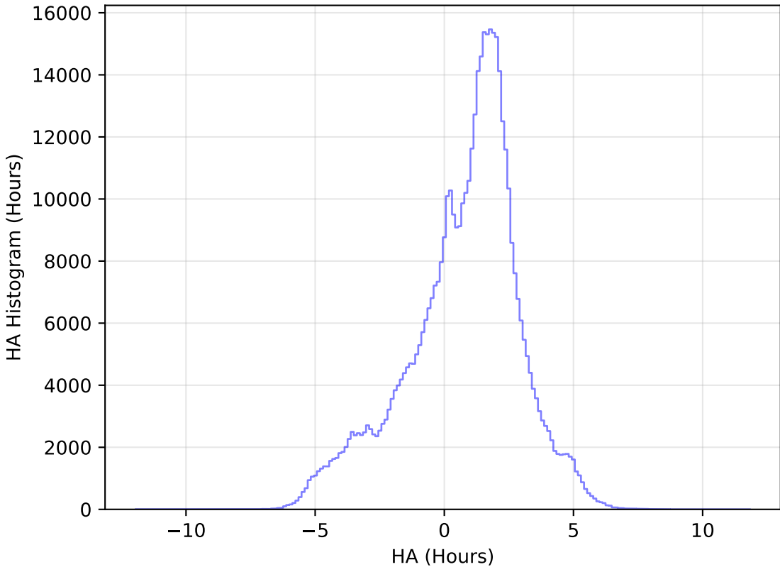
too_elab_heavy_r64_d2_ugrizy_v3.4_10yrs All sky i band: HA Histogram
