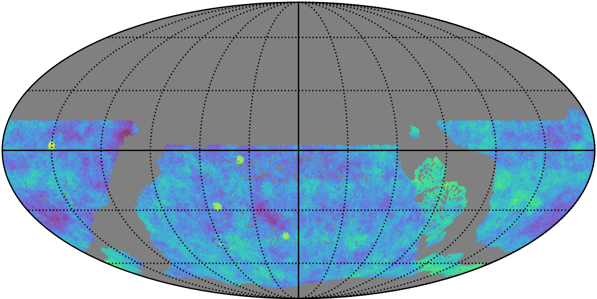
too_elab_heavy_r64_d2_ugrizy_v3.4_10yrs gri WFD: Fraction of visits in pairs (20-90 min)
