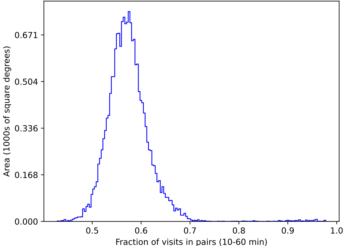
too_elab_heavy_r64_d2_ugrizy_v3.4_10yrs gri WFD: Fraction of visits in pairs (10-60 min)
