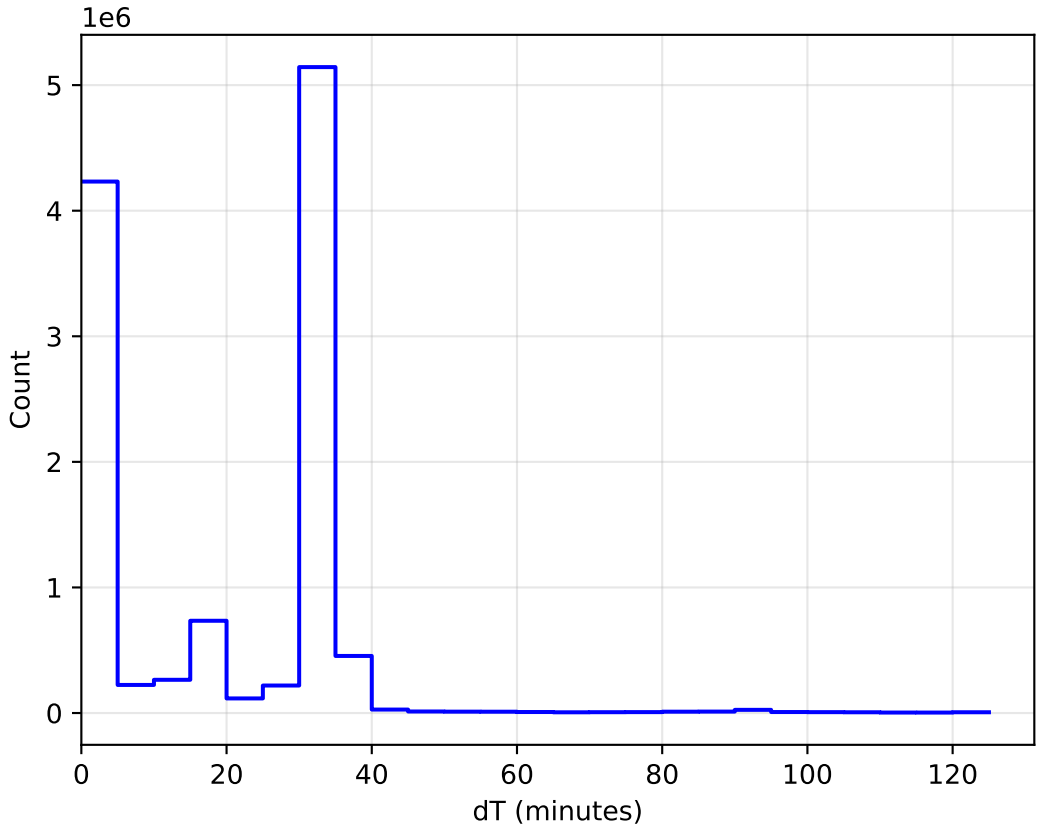
too_elab_heavy_r64_d2_ugrizy_v3.4_10yrs WFD: DeltaT Histogram
